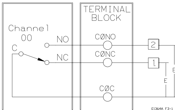
Figure 3-1. Example: Voltage Switching
